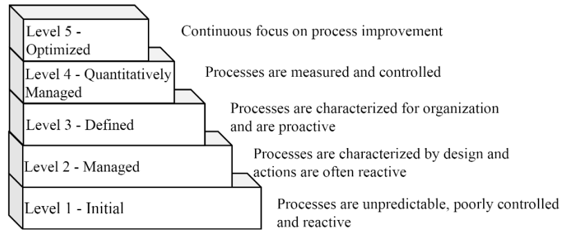
Figure 2. CMMI Levels.
